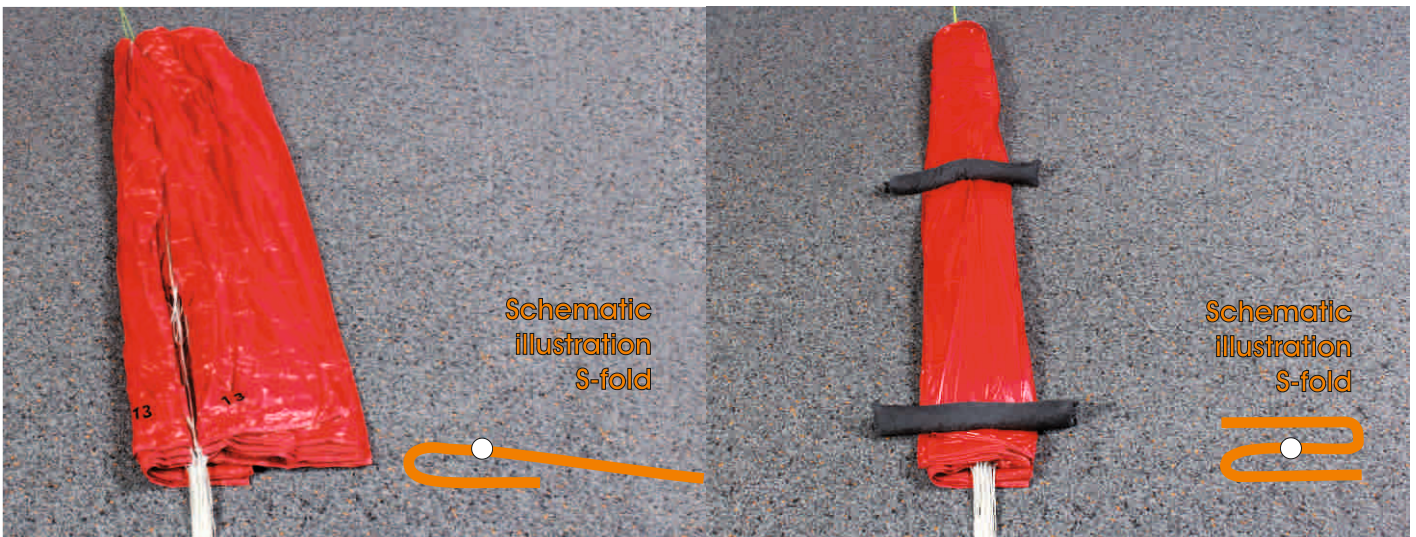
17. Fold right side S-shaped. (Step 1).
