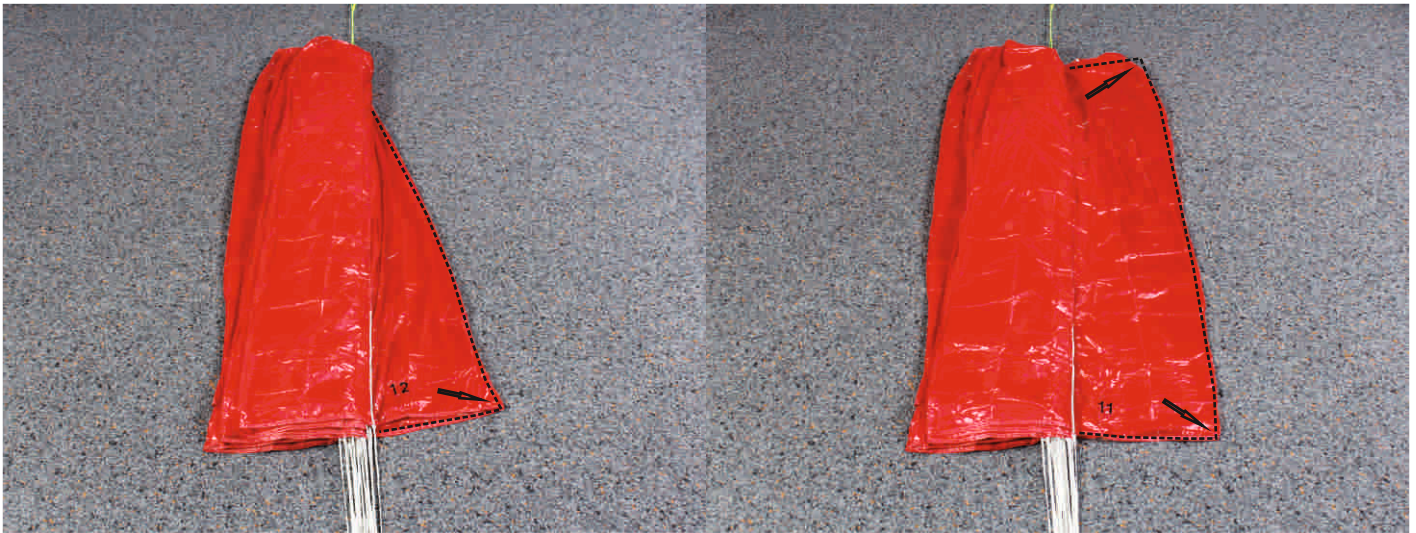
3. Place panel 13 (Cornetto 100: 11) centered to the floor and arrange panel 12 (Cornetto 100: 10) to the side.
