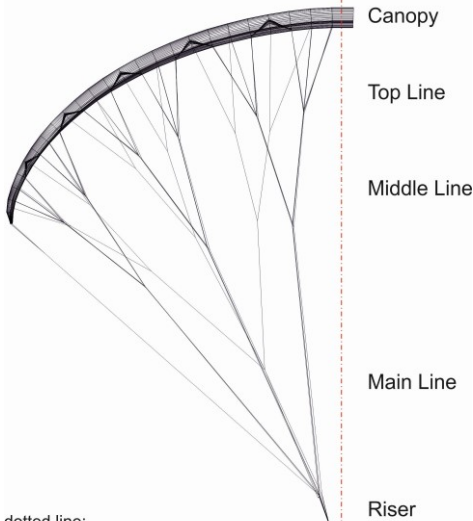
Fig. 1 CAD drawing of TWIN RS 2
