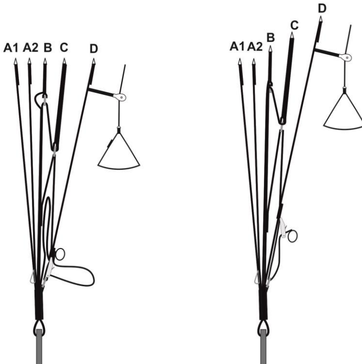
Fig. 6: TWIN RS risers showing how the trimmers work
