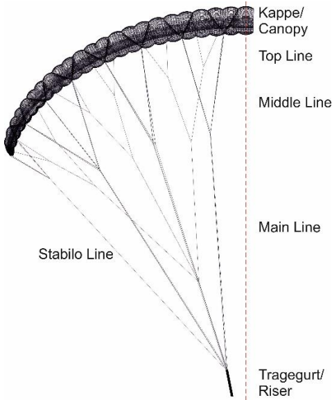
Fig. 1: CAD drawing of Astral 7
