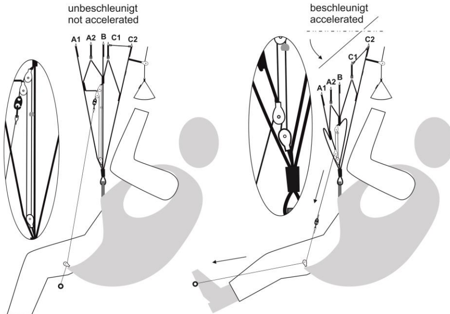
Fig. 5: How the Nexus speed system works
