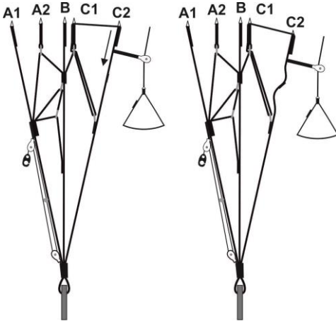
Fig. 8 Stabilizing by C-bridge
