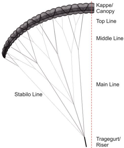
Fig. 1: CAD drawing of Sensis
