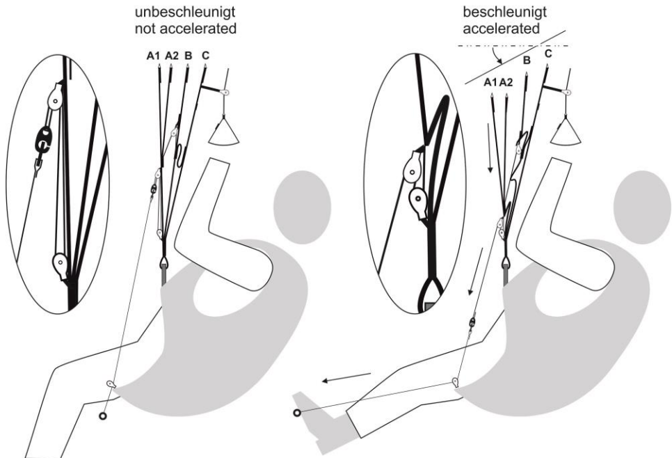
Fig. 5: How the Sensis speed system works
