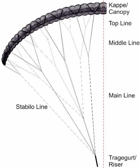
Fig. 1: CAD drawing of Nyos
