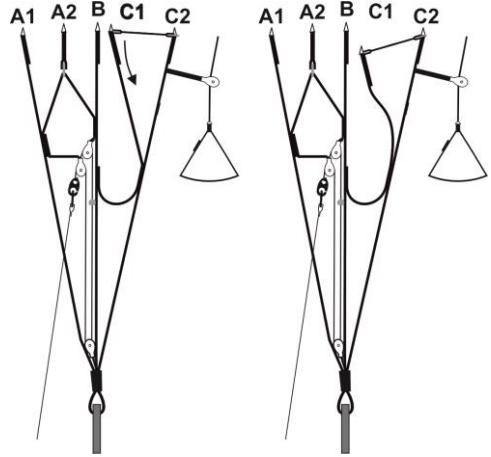
Fig. 7: Adjustment of flightdirection by C-bridge
