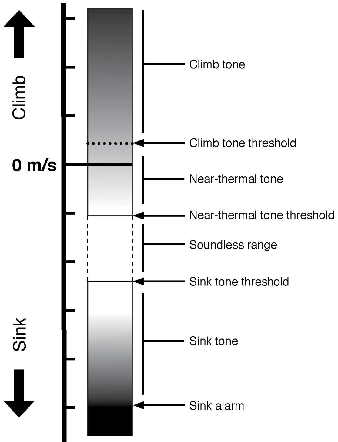
The various tones for the Element vario.
